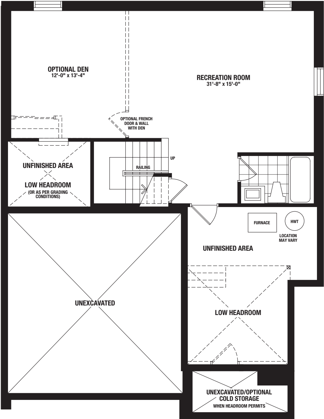
FINISHED BASEMENT - ELEVATION A
