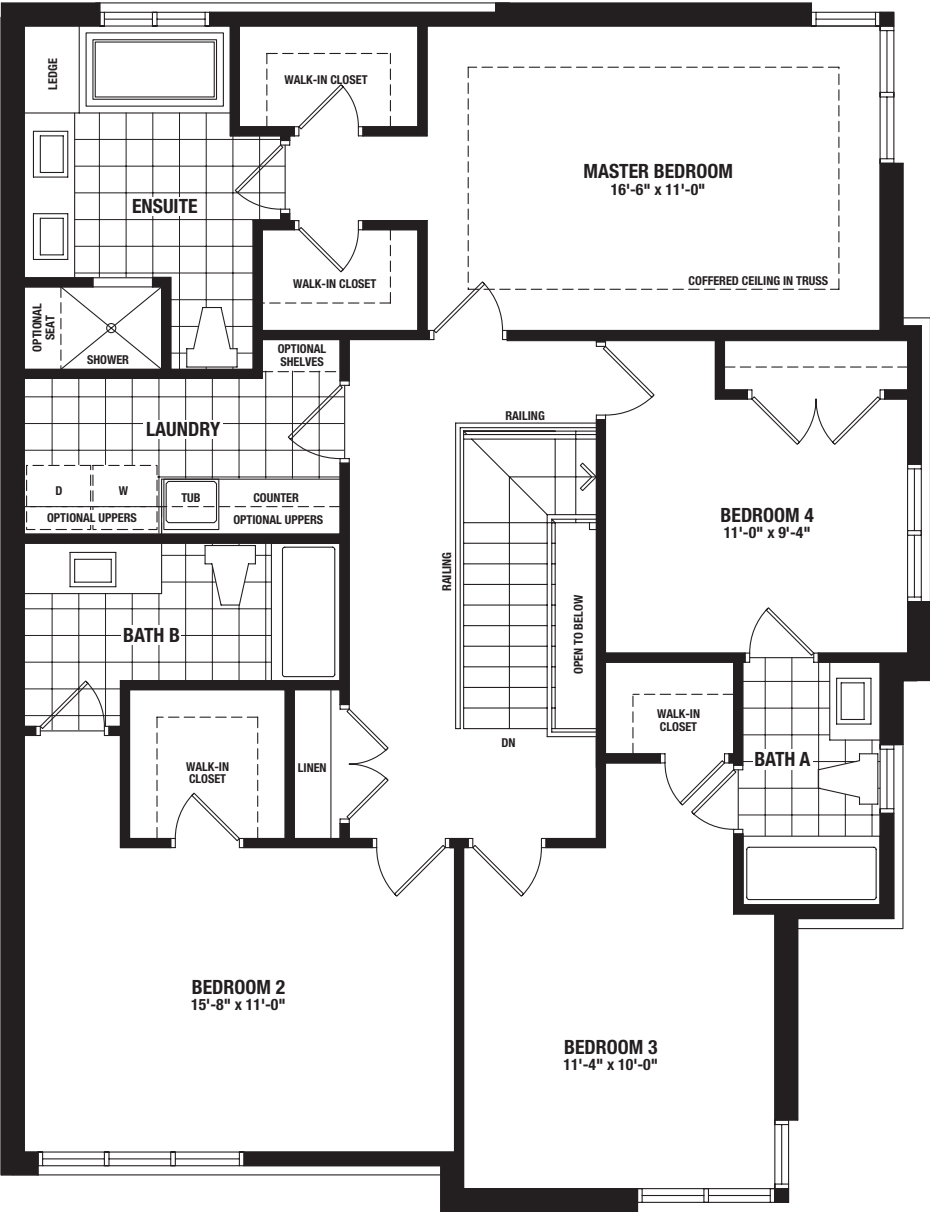
SECOND FLOOR - ELEVATION B
