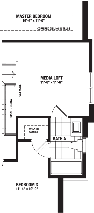
PARTIAL SECOND FLOOR OPTIONAL MEDIA LOFT - ELEVATION B
