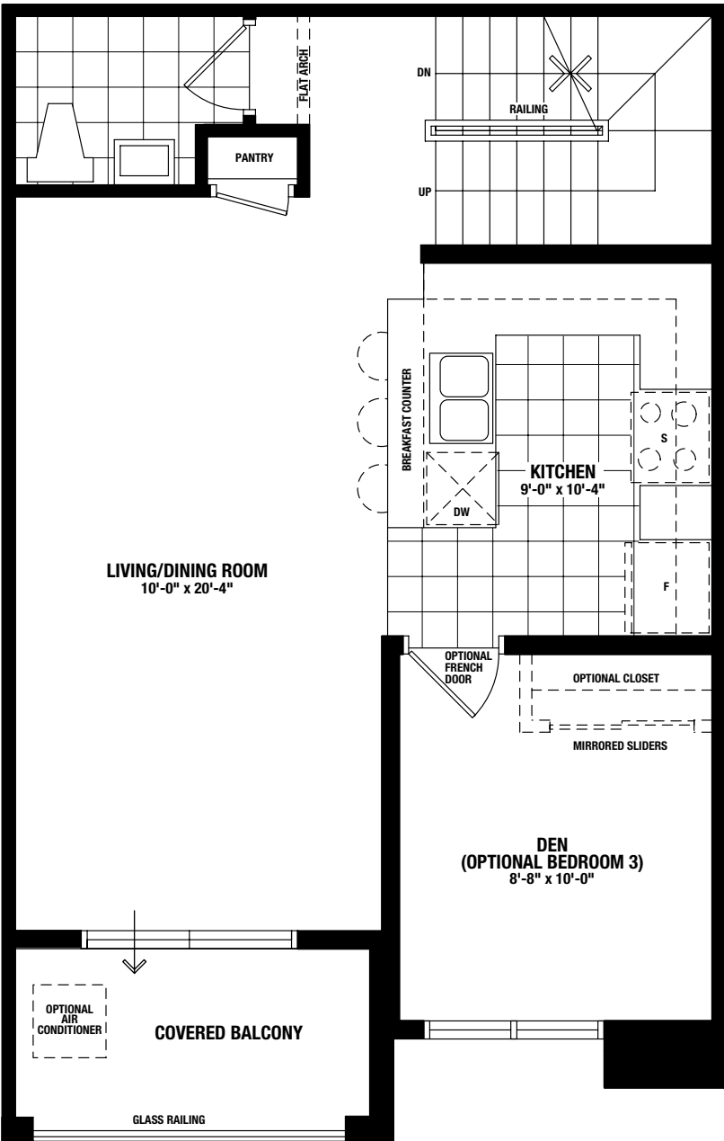
MAIN FLOOR - ELEVATION A
