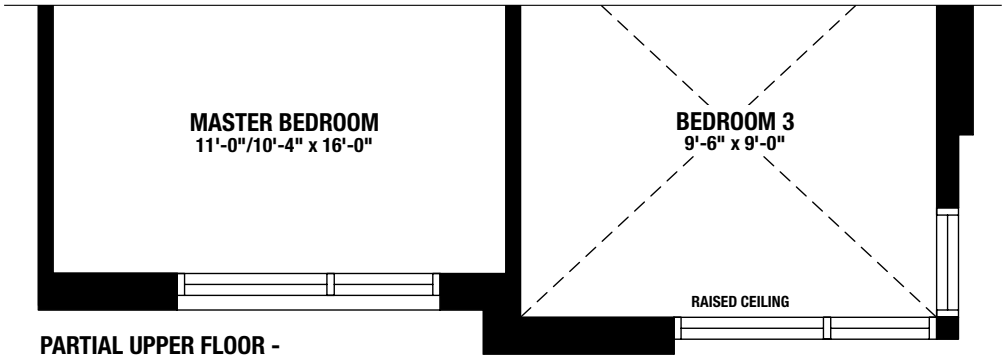
PARTIAL UPPER FLOOR - ELEVATION B
