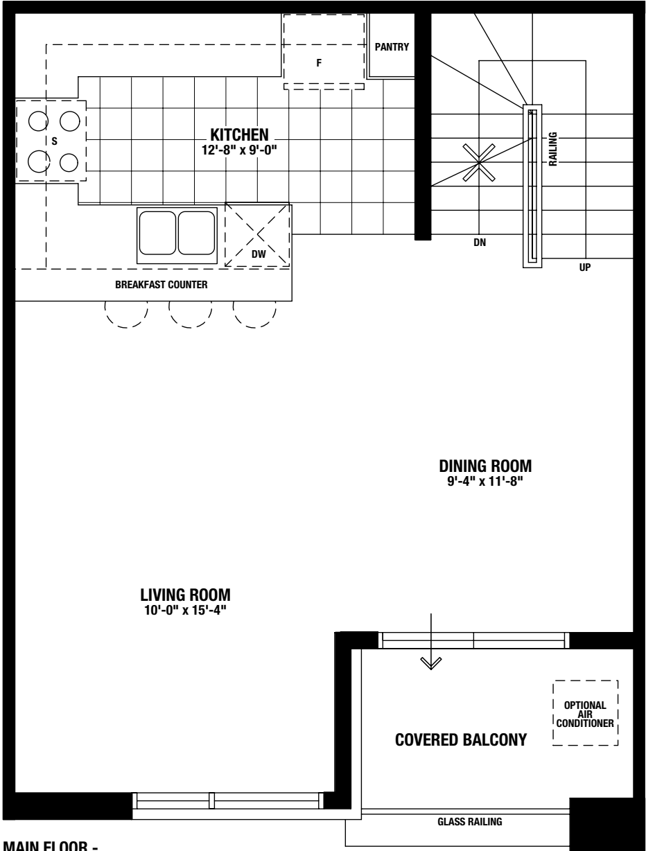
MAIN FLOOR - ELEVATION A
