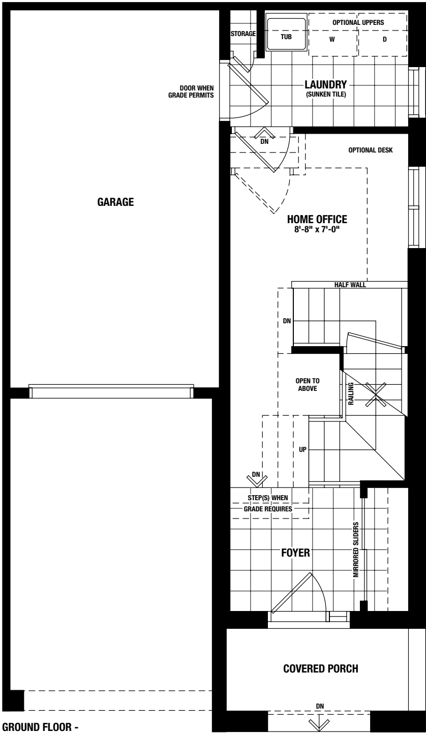
GROUND FLOOR - ELEVATION A & B
