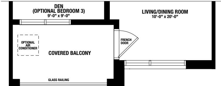
PARTIAL MAIN FLOOR - ELEVATION B
