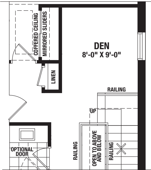
PARTIAL SECOND FLOOR OPTIONAL DEN LAYOUT ELEVATION A & B
