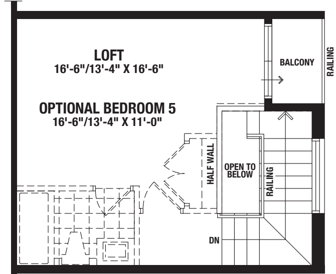
FINISHED LOFT - ELEVATION A & B
