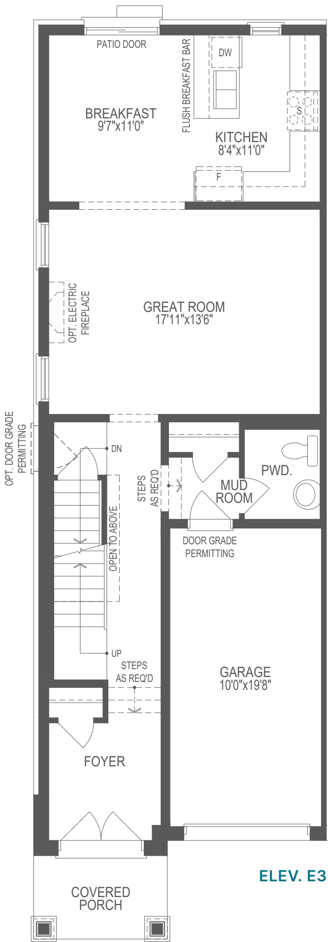
PARTIAL GROUND FLOOR WITH ALTERNATE POWDER ROOM
