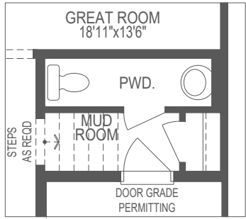
PARTIAL GROUND FLOOR WITH ALTERNATE POWDER ROOM
