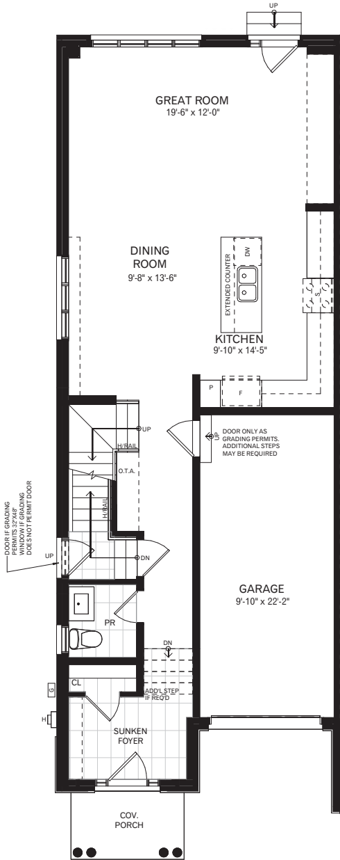
GROUND FLOOR
