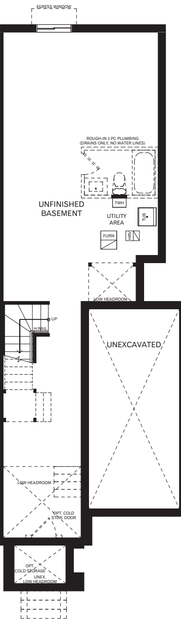
BASEMENT
