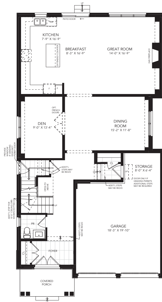
GROUND FLOOR A
