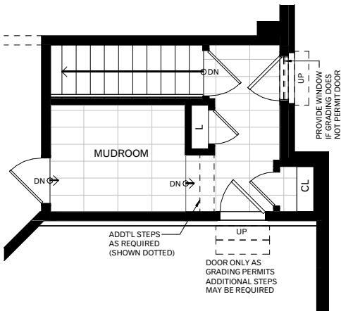
Partial Ground Floor Plan With Opt. Mudroom In Lieu Of Laundry
