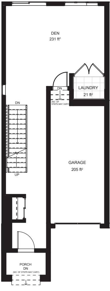
GROUND LEVEL
