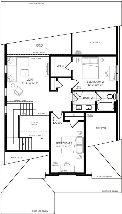
SECOND FLOOR PLAN A
