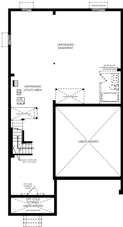
BASEMENT PLAN A
