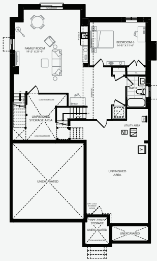
OPTIONAL FINISHED BASEMENT PLAN WALKOUT + 960 Sq. Ft.
