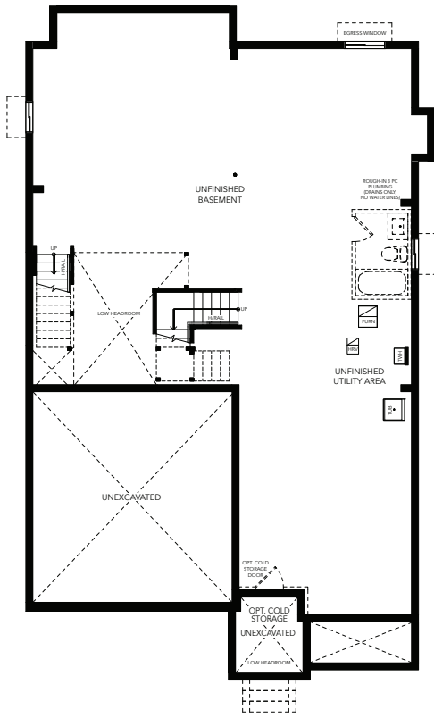
BASEMENT PLAN A
