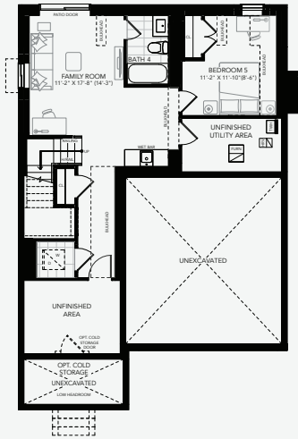
OPTIONAL FINISHED BASEMENT PLAN WALKOUT + 650 Sq. Ft.
