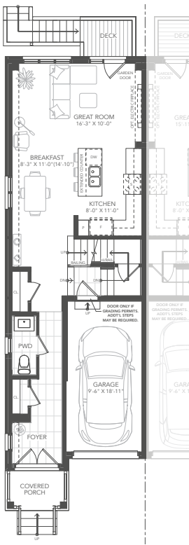
GROUND FLOOR PLAN A
