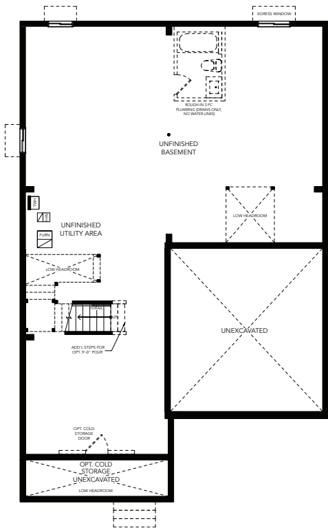
BASEMENT PLAN A
