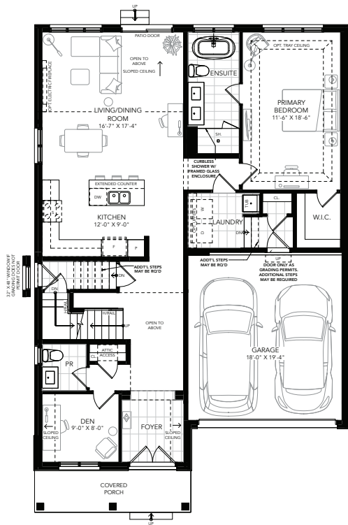
GROUND FLOOR PLAN A
