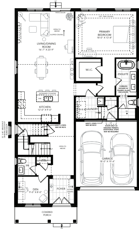
GROUND FLOOR PLAN A
