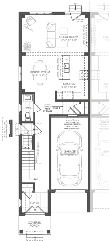
GROUND FLOOR PLAN A
