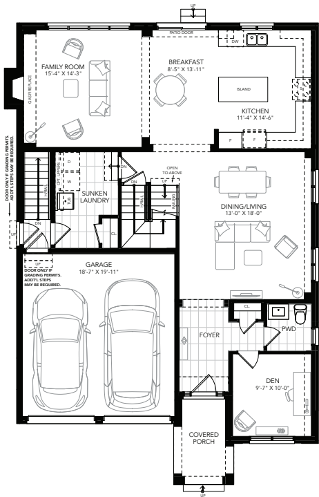
GROUND FLOOR PLAN A
