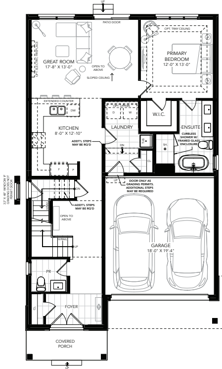
GROUND FLOOR PLAN A
