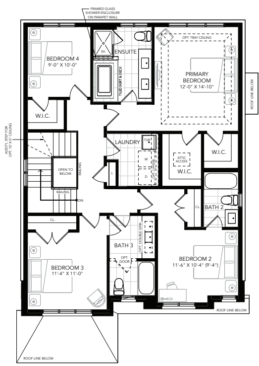
SECOND FLOOR PLAN A
