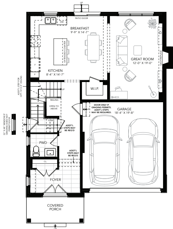
GROUND FLOOR PLAN A
