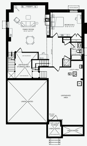
OPTIONAL FINISHED BASEMENT PLAN + 960 Sq. Ft.
