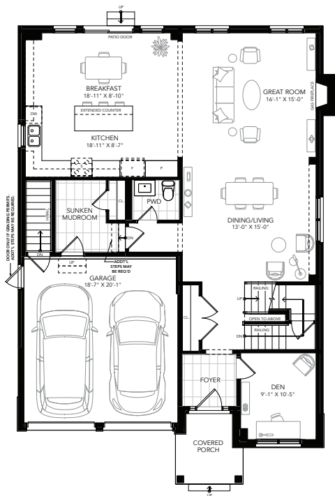
GROUND FLOOR PLAN A
