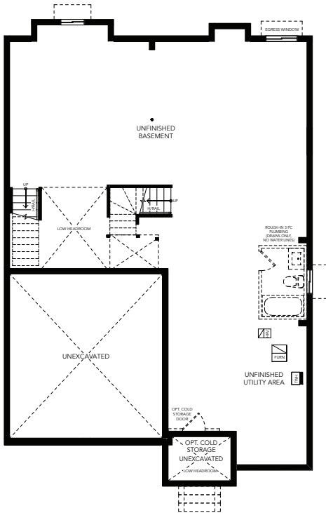
BASEMENT PLAN A
