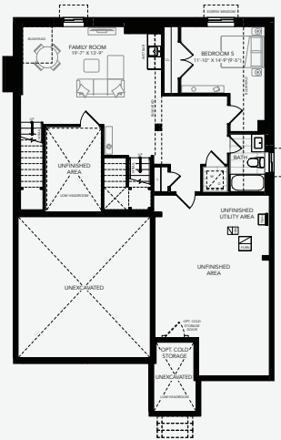
OPTIONAL FINISHED BASEMENT PLAN + 790 Sq. Ft.
