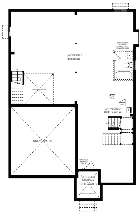
BASEMENT PLAN A
