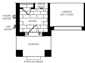
ELEVATION B Ground Floor
