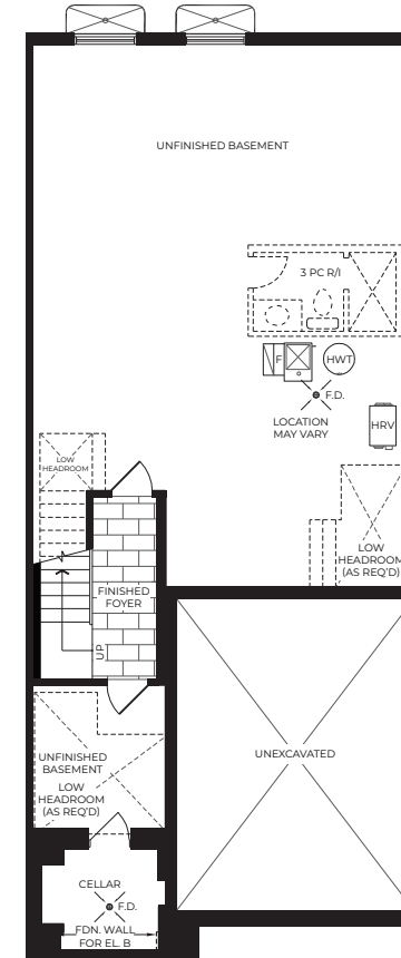
ELEVATION A & B Basement
