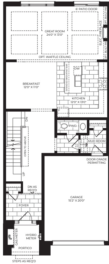
ELEVATION A Ground Floor
