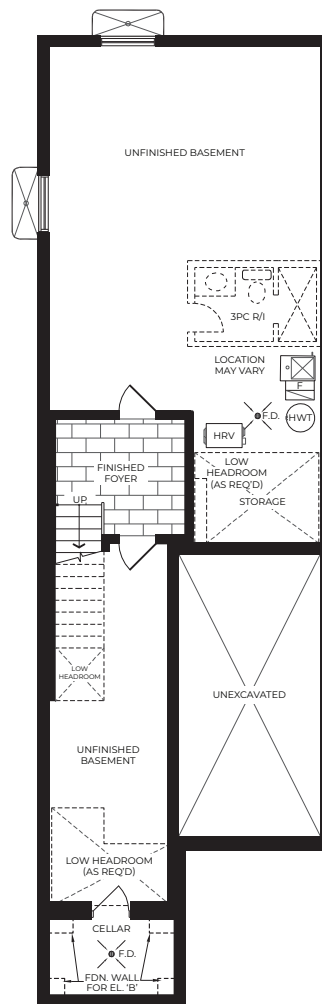
ELEVATION A & B Basement
