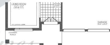
PARTIAL GROUND FLOOR STYLE C
