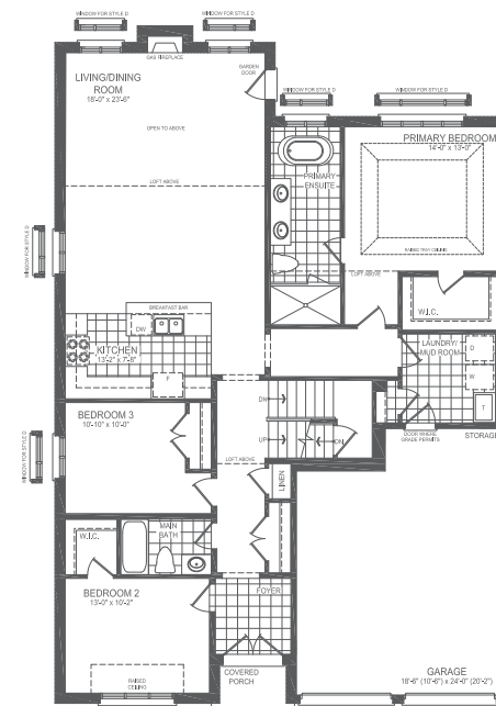
OPT. GROUND FLOOR STYLE A FOR LOFT
