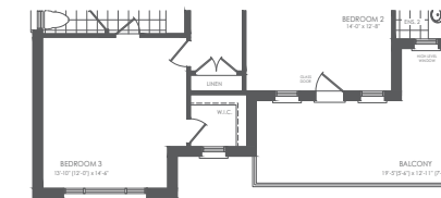
PARTIAL SECOND FLOOR STYLE D
