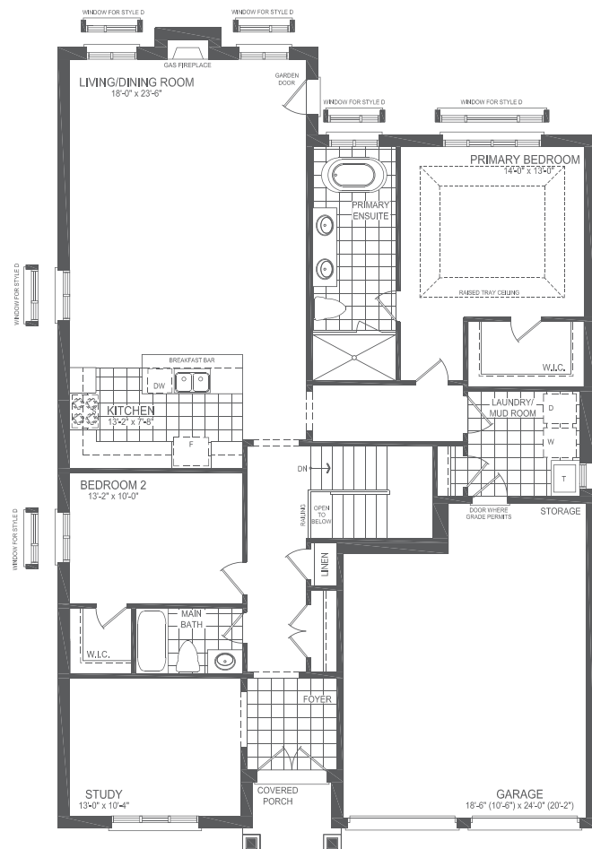
GROUND FLOOR STYLE A FOR NON-LOFT
