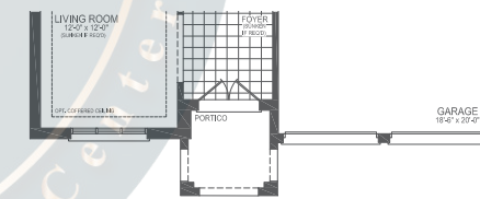
PARTIAL GROUND FLOOR STYLE B
