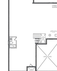
BASEMENT STYLE A / C FOR LOFT
