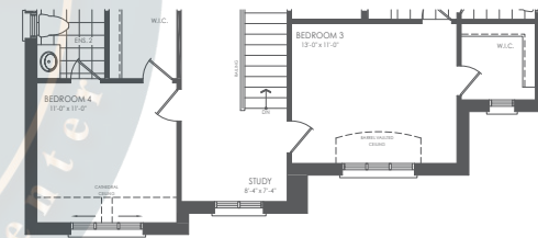
PARTIAL SECOND FLOOR STYLE B
