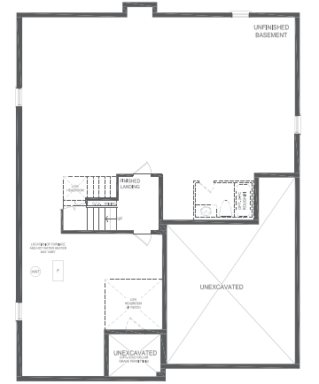
BASEMENT STYLE A FOR NON-LOFT
