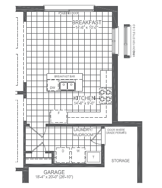
PARTIAL GROUND FLOOR FOR OPT. 5 BEDROOM SECOND FLOOR STYLE A/B/C/D
