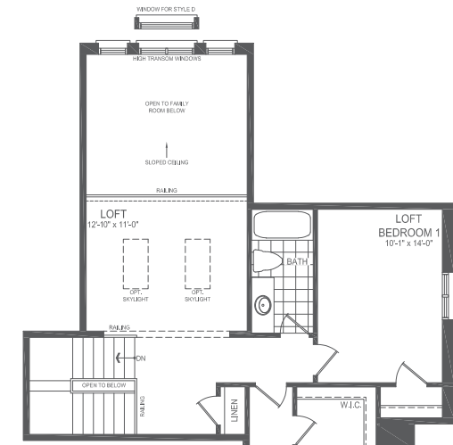
LOFT FLOOR STYLE A
