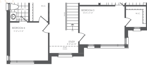
PARTIAL SECOND FLOOR STYLE D
