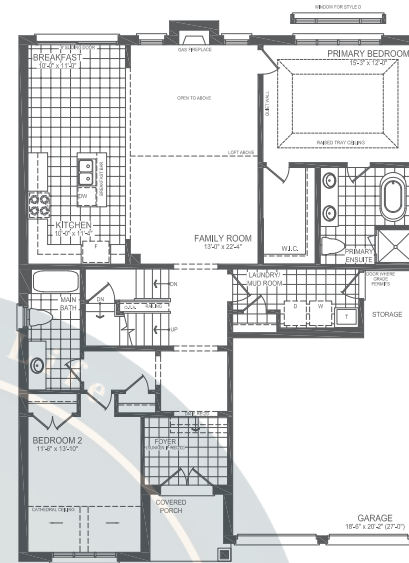
GROUND FLOOR STYLE A FOR LOFT
