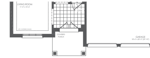
PARTIAL GROUND FLOOR STYLE B
