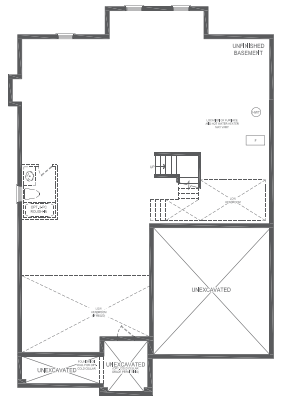
PARTIAL BASEMENT FOR OPT. GROUND FLOOR IN-LAW SUITE STYLE A
