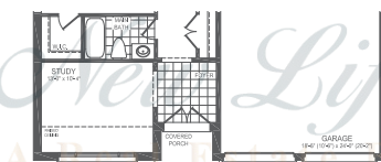
PARTIAL GROUND FLOOR STYLE D FOR NON-LOFT
