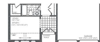
PARTIAL GROUND FLOOR STYLE C FOR LOFT AND NON-LOFT
