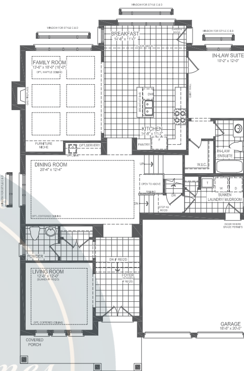
OPT. GROUND FLOOR IN-LAW SUITE STYLE A
