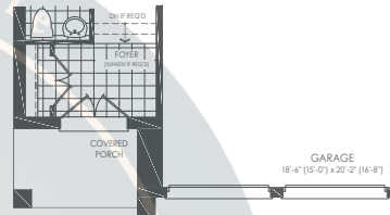
PARTIAL GROUND FLOOR STYLE E
