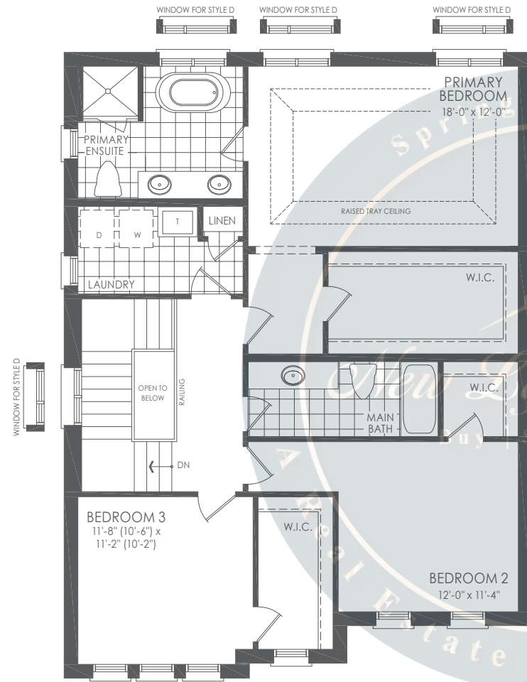
SECOND FLOOR STYLE B
