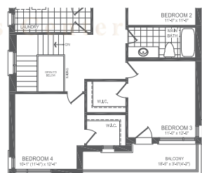
PARTIAL SECOND FLOOR STYLE E
