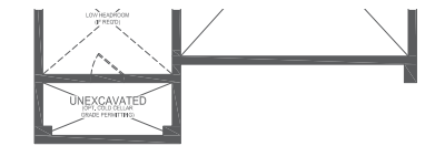
PARTIAL BASEMENT STYLE E
