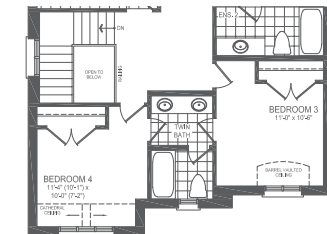
PARTIAL OPT. 3 BATH SECOND FLOOR STYLE C
