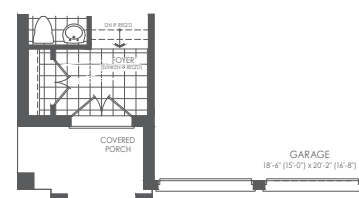
PARTIAL GROUND FLOOR STYLE D
