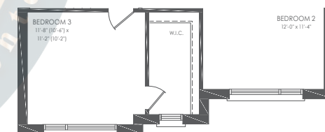
PARTIAL SECOND FLOOR STYLE D
