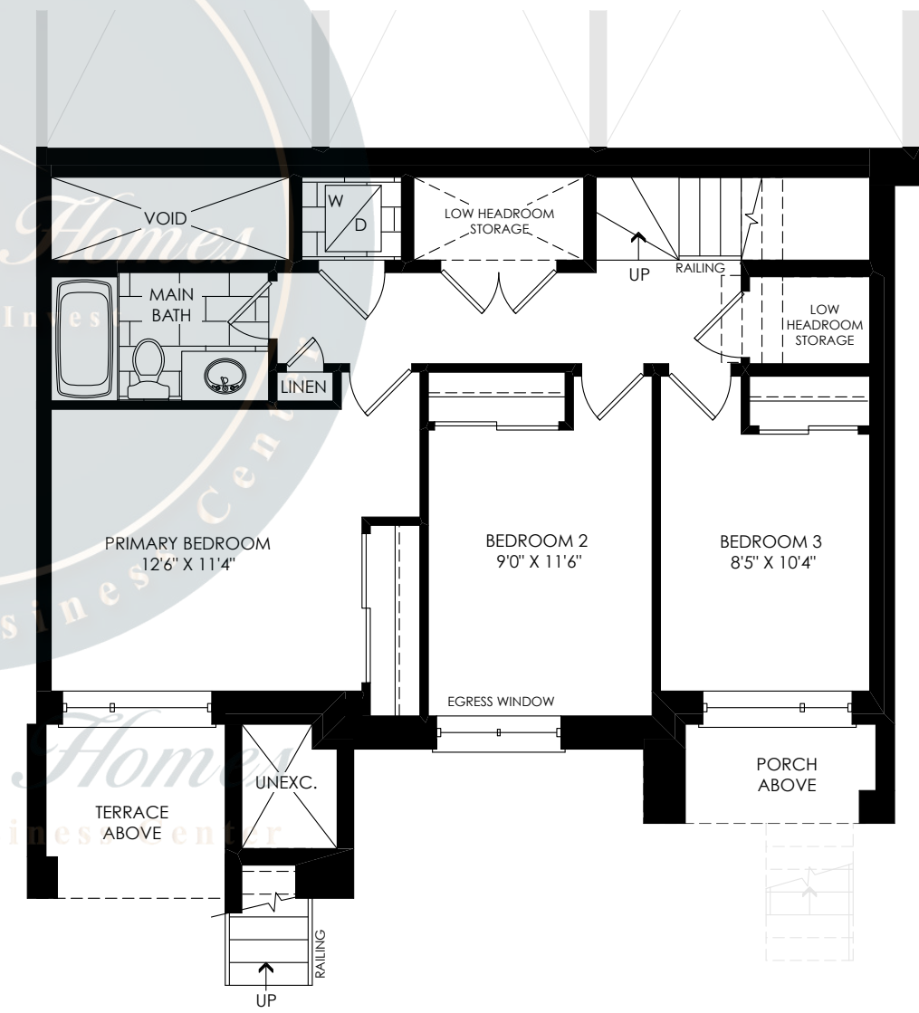
EXTERIOR END LOWER FLOOR PLAN (FRONT)
