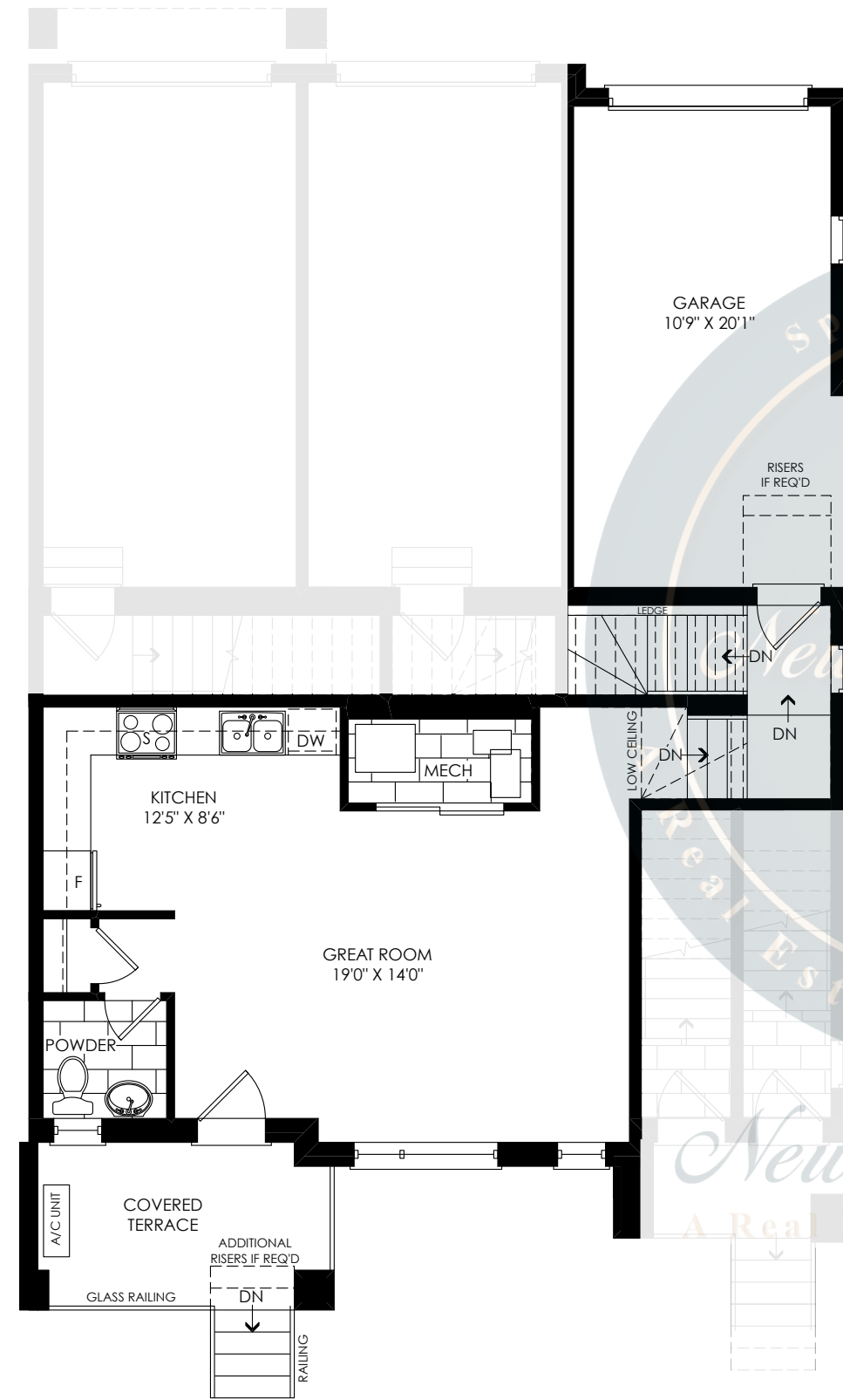
EXTERIOR END MAIN FLOOR PLAN (FRONT)
