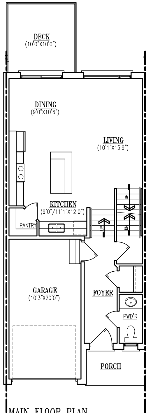
MAIN FLOOR PLAN INTERIOR UNIT 618 SQ. FT. 1494 SQ. FT. TOTAL
