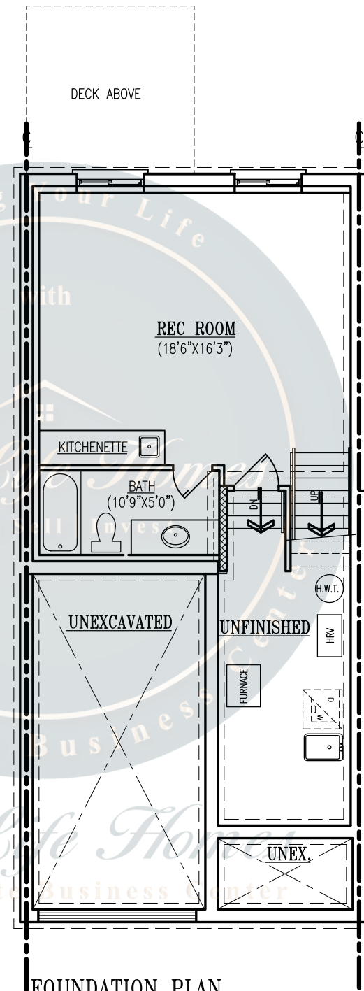
FOUNDATION PLAN INTERIOR UNIT 384 SQ. FT. FINISHED
