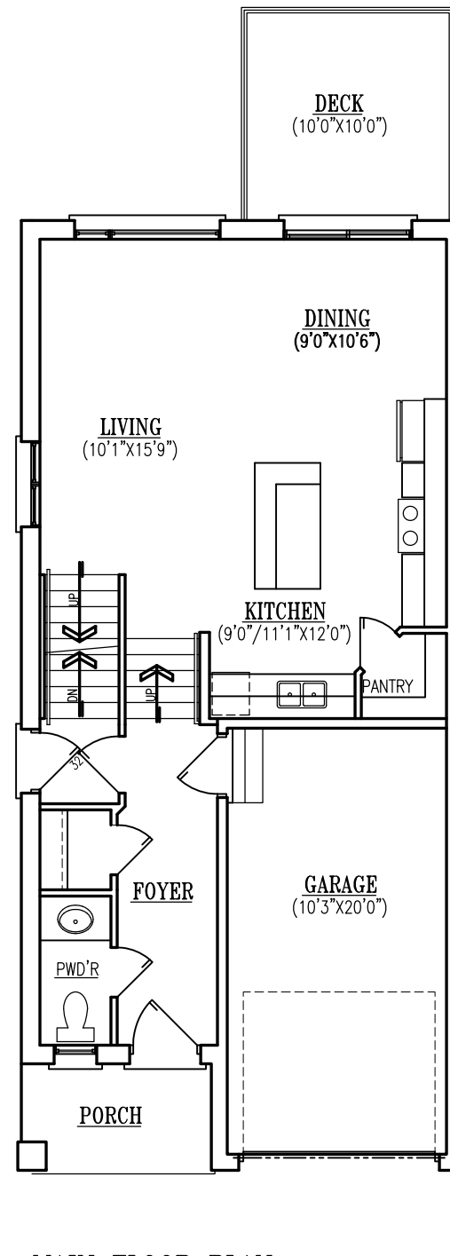
MAIN FLOOR PLAN CORNER UNIT 624 SQ. FT. 1508 SQ. FT. TOTAL
