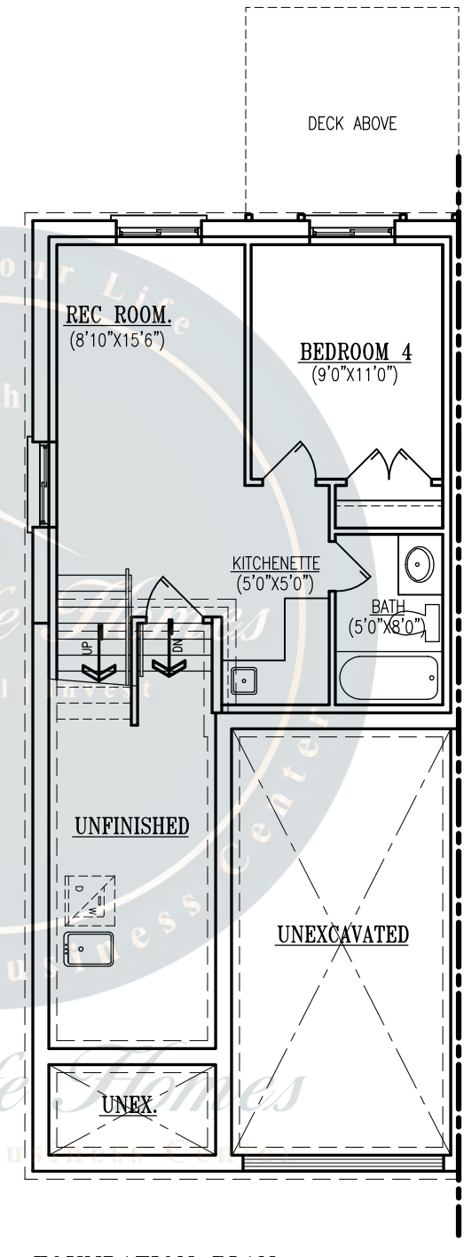
FOUNDATION PLAN CORNER UNIT 384 SQ. FT. FINISHED
