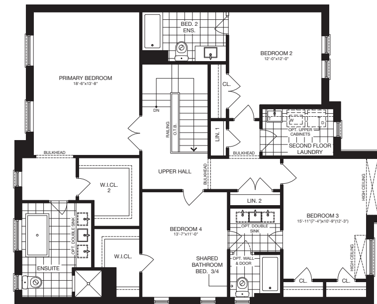
SECOND FLOOR (ELEV. A) - 4 BEDROOM + ENSUITE
