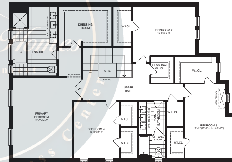
SECOND FLOOR (ELEV. A) - 4 BEDROOM
