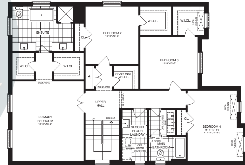
SECOND FLOOR (ELEV. A) - 4 BEDROOM
