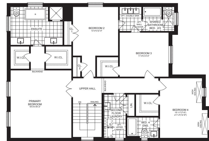
SECOND FLOOR (ELEV. A) - 4 BEDROOM + ENSUITE
