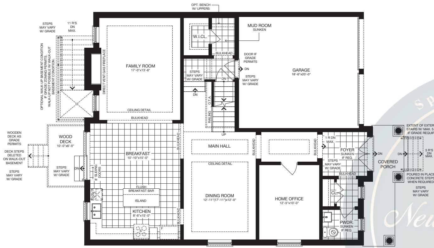
GROUND FLOOR (ELEV. A)
