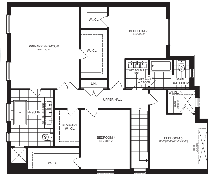
SECOND FLOOR (ELEV. A) - 4 BEDROOM
