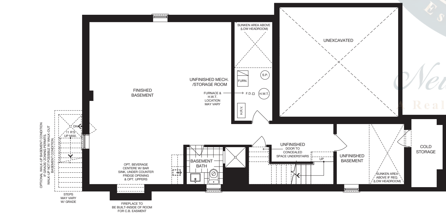
OPTIONAL FINISHED BASEMENT (ELEV. A)
