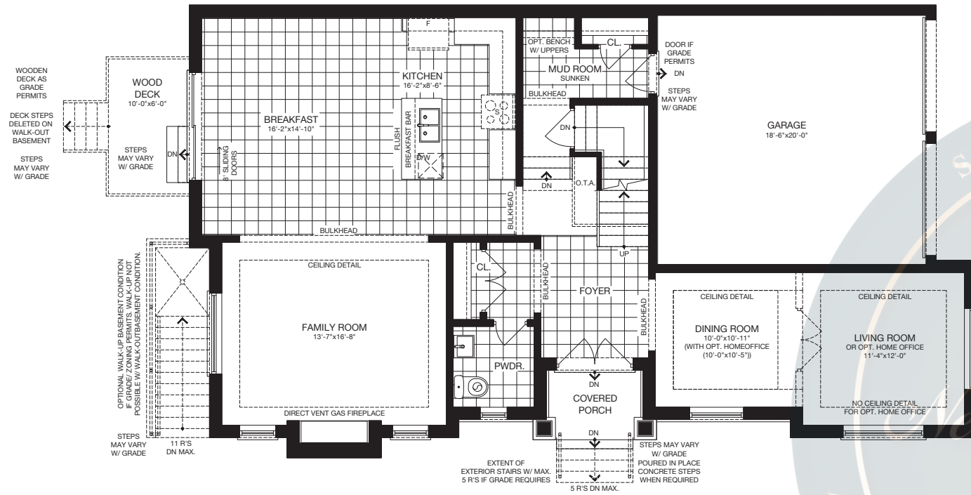
GROUND FLOOR (ELEV. A)
