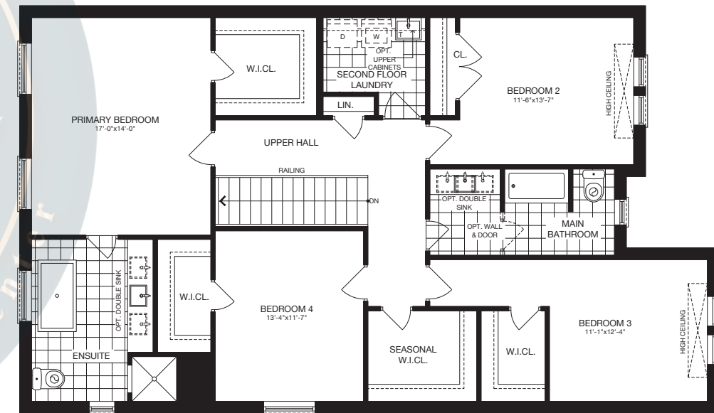
SECOND FLOOR (ELEV. A) - 4 BEDROOM
