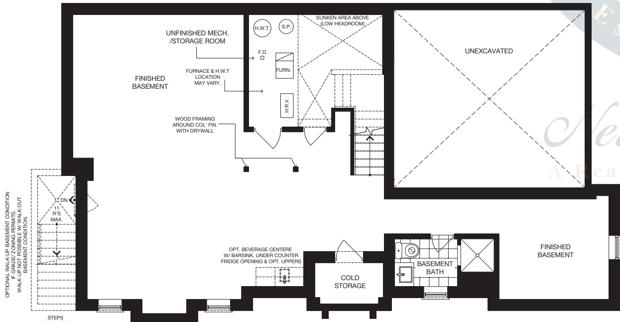
OPTIONAL FINISHED BASEMENT (ELEV. A)
