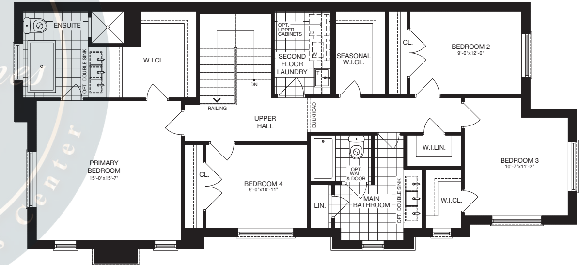
SECOND FLOOR (ELEV. A) - 4 BEDROOM
