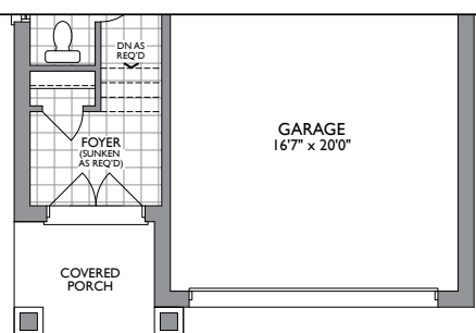
PARTIAL MAIN LEVEL ELEV. B & C
