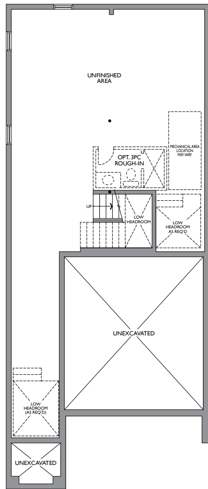
LOWER LEVEL ELEV. A, B & C
