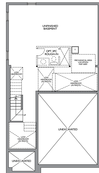
LOWER LEVEL ELEV. A, B & C
