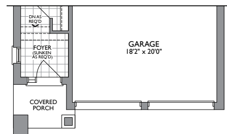
PARTIAL MAIN LEVEL ELEV. C
