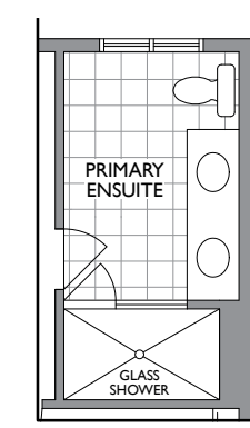
PARTIAL UPPER LEVEL ALT. ENSUITE ELEV. A
