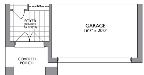
PARTIAL MAIN LEVEL ELEV. C
