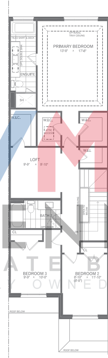
Second Floor - Elevation C
