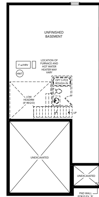
ELEVATION A & B | LOWER LEVEL
