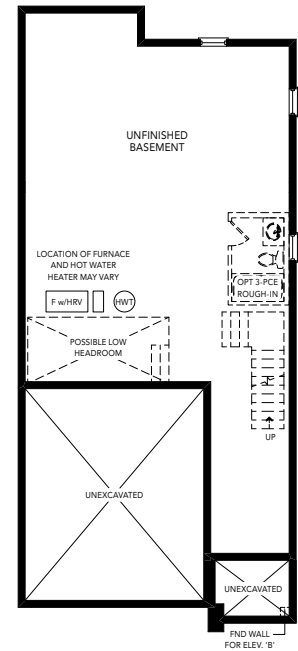
ELEVATION A & B | LOWER LEVEL
